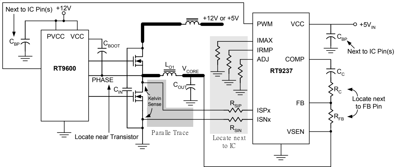
Figure 8. Layout Consideration
